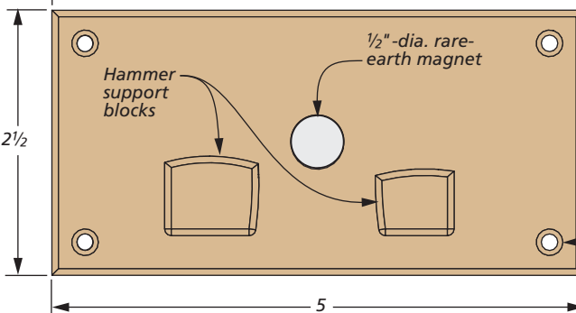
HAMMER HOLDER FRONT VIEW
