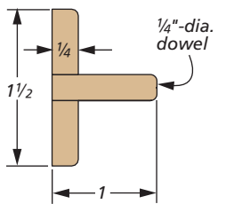
END SECTION VIEW
