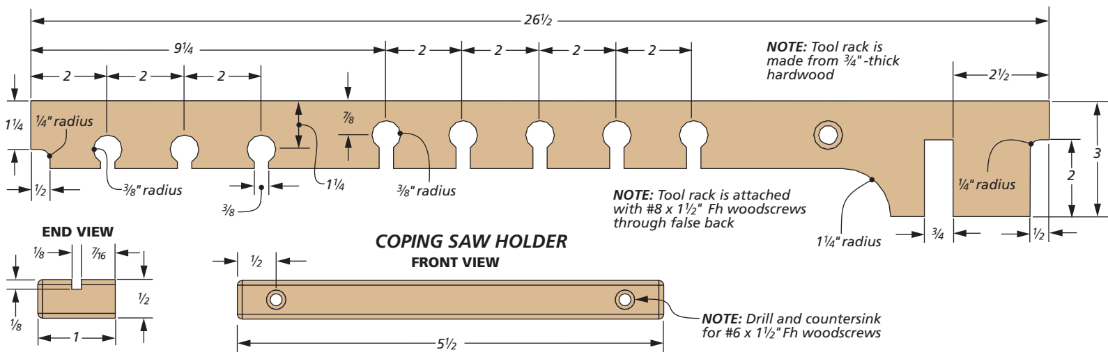
TOOL RACK TOP VIEW
