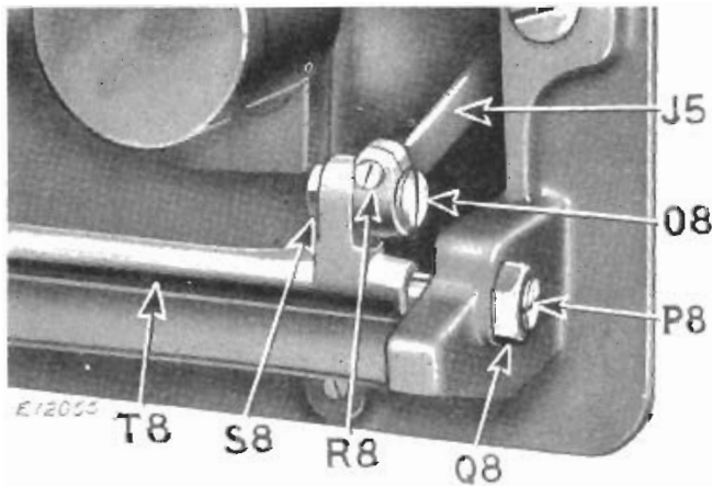
FIG. 41. LENGTHWISE ADJUSTMENT OF FEED DOG
