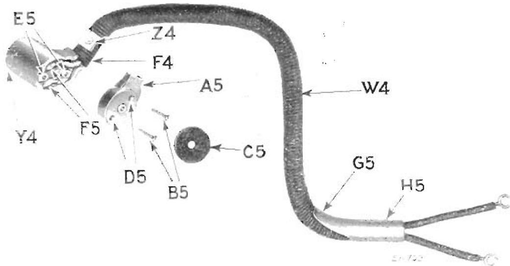
FIG. 9. SINGERLIGHT DISASSEMBLED LEADS REMOVED FROM MACHINE 201-2
