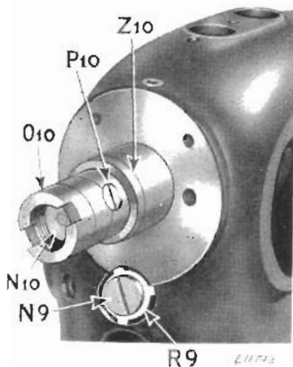
FIG. 56 TO REMOVE FEED REGULATOR
