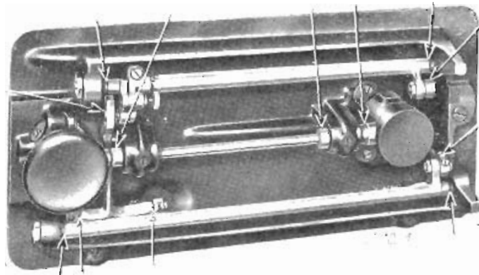
FIG. 67. OILING POINTS IN BASE OF MACHINE
