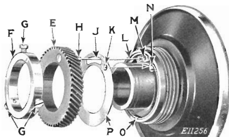
FIG. 19. BALANCE WHEEL DISASSEMBLED (MACHINE 201 2)
