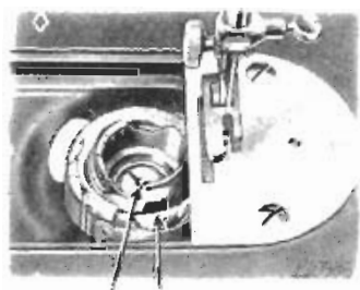
FIG. 65 VIEW OF SEWING HOOK SHOWING OILING POINTS
