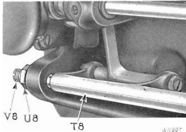
FIG. 42. SIDEWISE ADJUSTMENT OF FEED DOG
