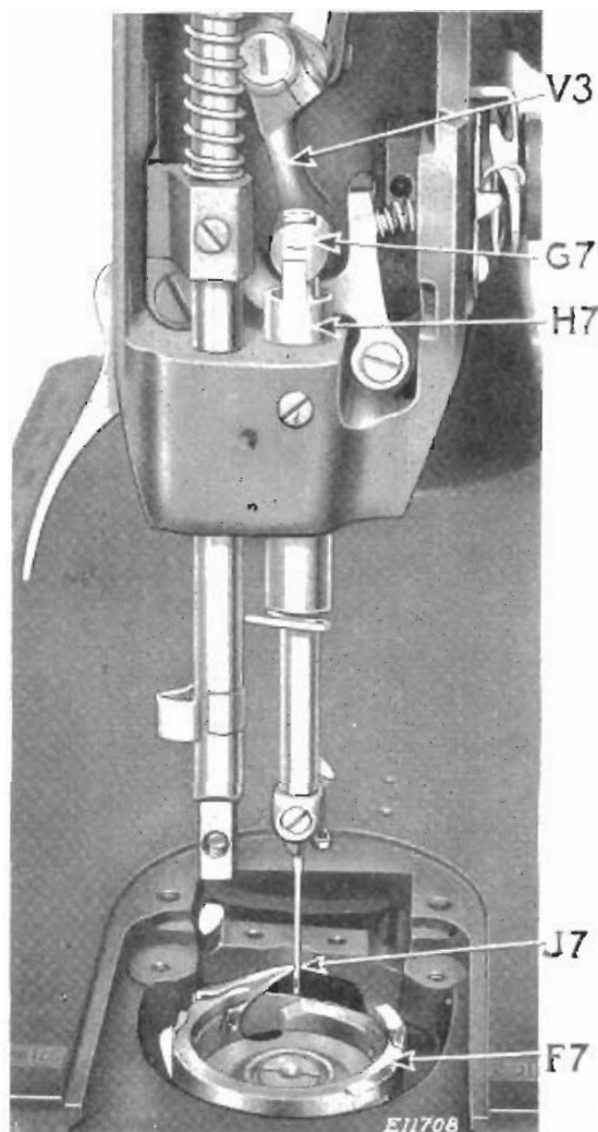
FIG. 33. NEEDLE BAR AND ROTATING HOOK CORRECTLY TIMED
