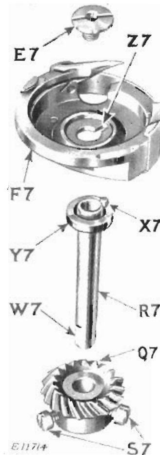
FIG. 37. ROTATING HOOK SHAFT AND GEAR (REMOVED AND DISASSEMBLED)
