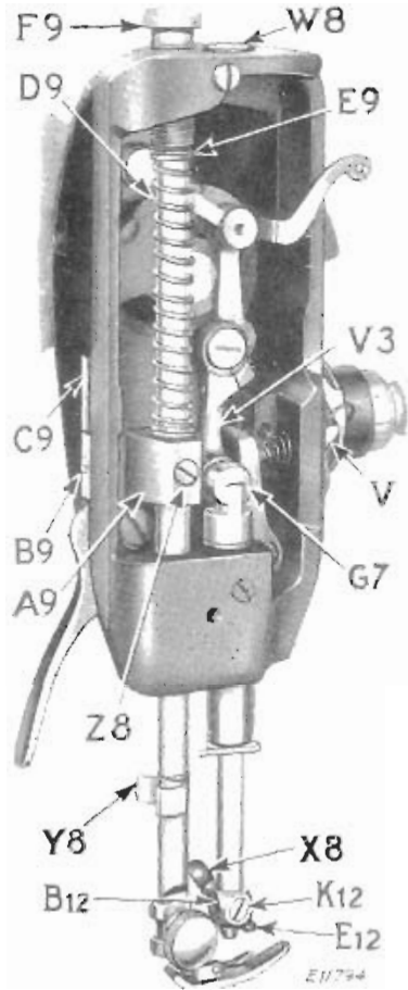
FIG. 52. To REMOVE NEEDLE BAR AND PRESSER BAR
