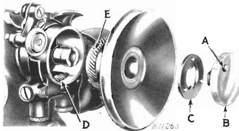
FIG. 18. BALANCE WHEEL REMOVED (MACHINE 201-2)
