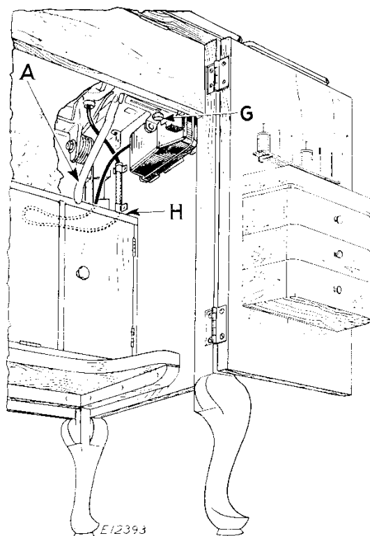
FIG. 6. BAKELITE CONTROLLER ARRANGED FOR KNEE CONTROL IN CABINET 48
