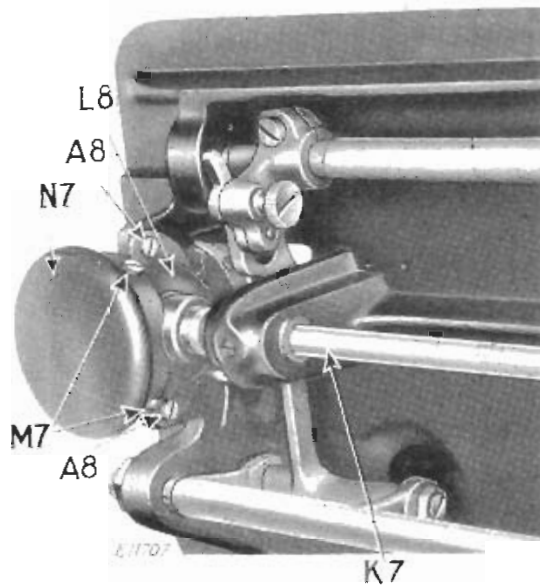
FIG. 34. REMOVING ROTATING HOOK SHAFT BEVEL GEAR COVER
