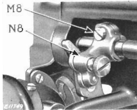
FIG. 40. TO RAISE OR LOWER THE FEED DOG
