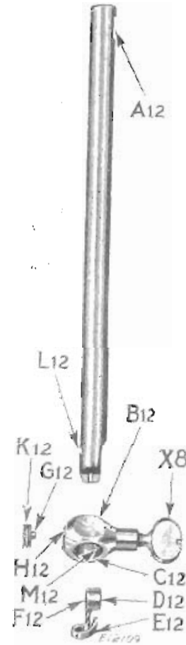
FIG. 52A. NEEDLE BAR REMOVED AND DISASSEMBLED
