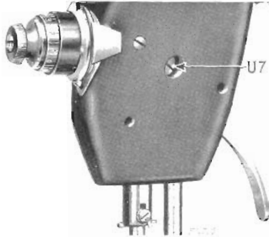
FIG. 36. SCREW TO ADJUST NEEDLE BAR HEIGHT
