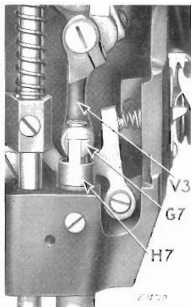
FIG. 32. CORRECT ADJUSTMENT OF TIMING GAUGE
