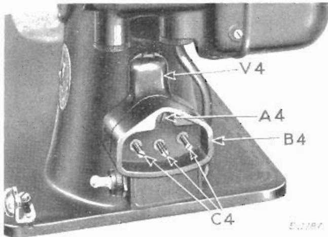
FIG. 7. THREE-PIN TERMINAL IN PLACE ON MACHINE 201-2
