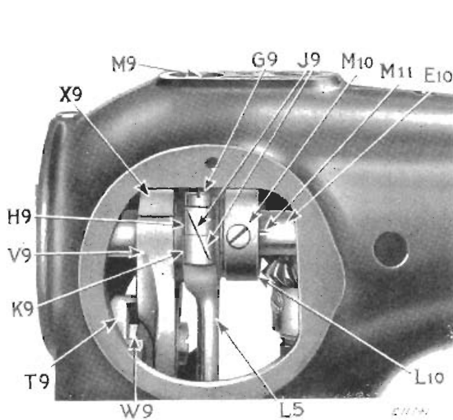
FIG. 53. To REMOVE FEED CONNECTING ROD
