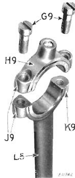
FIG. 54. FEED CONNECTING ROD REMOVED SHOWING UPPER END
