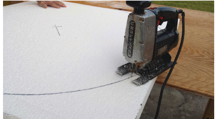
Figure 3. Use a jigsaw to cut along circle drawn on Styrofoam. Credits: Edmund L. Thralls, UF/IFAS
