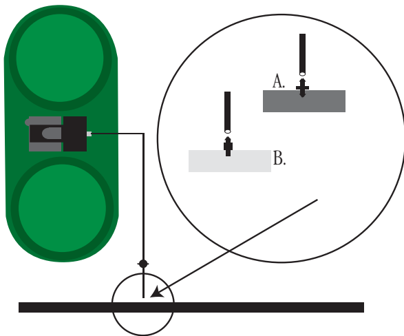
A. Rigid PVC pipe use 10/32" threaded joiners with teflon tape B. Soft Poly tubing use .16" double barb joiners w/ silicone sealant
