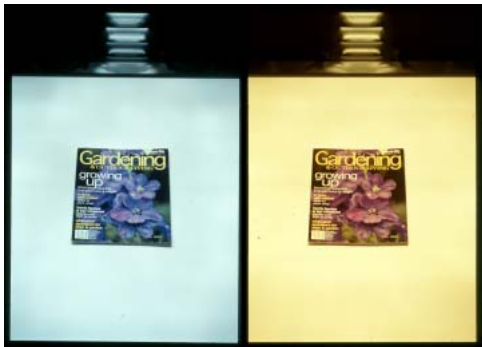
On the left is a Metal Halide lamp, notice the white/blue hue. The lamp on the right is a High Pressure Sodium and exhibits a warmer, yellow/orange hue.
