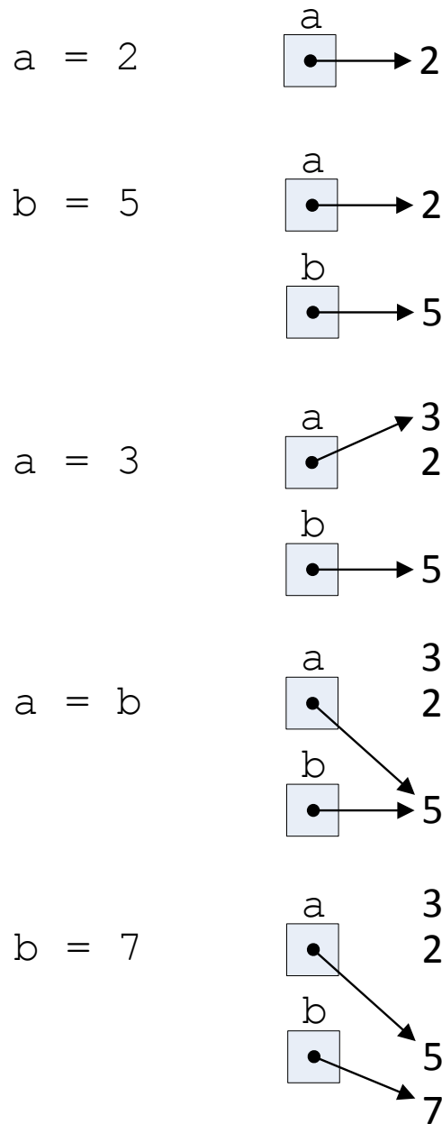
Figure 2.2: How variable bindings change as a program runs
