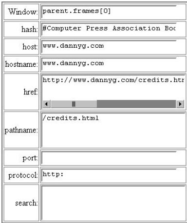
Figure 17-2: Readout of all window.location properties for the left frame
