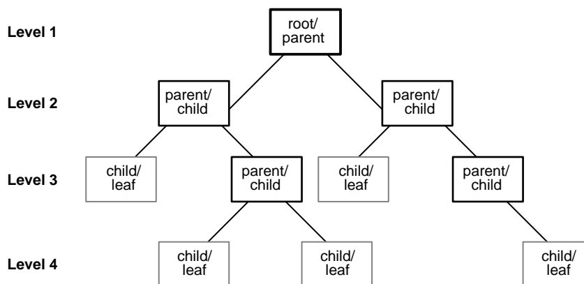
Figure 2–1 Hierarchical Tree
