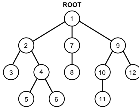
Figure 7-1 Hierarchical Queries
