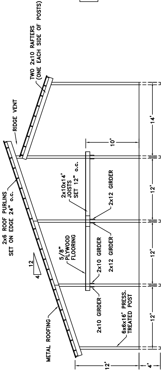
CROSS SECTION SCALE: 3/32"=1'-0"
