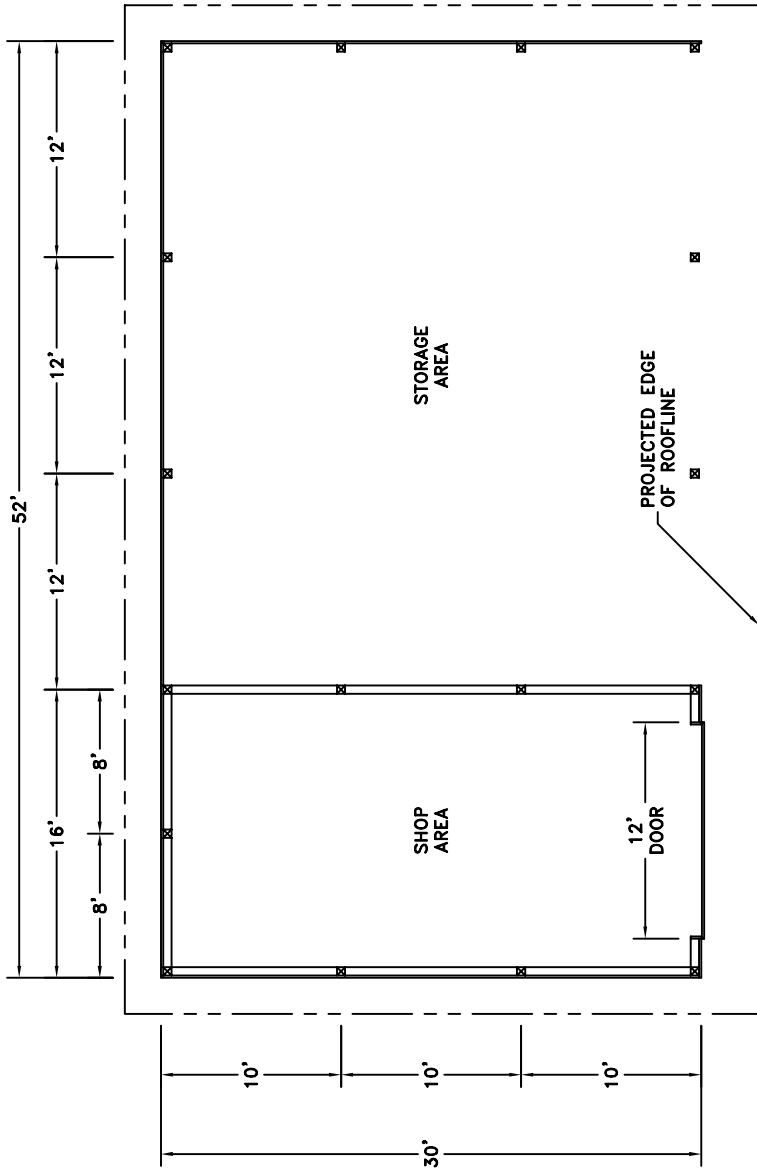
PLAN SCALE: 3/32"=1'-0"
